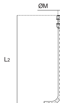
PERNOS Bolts
